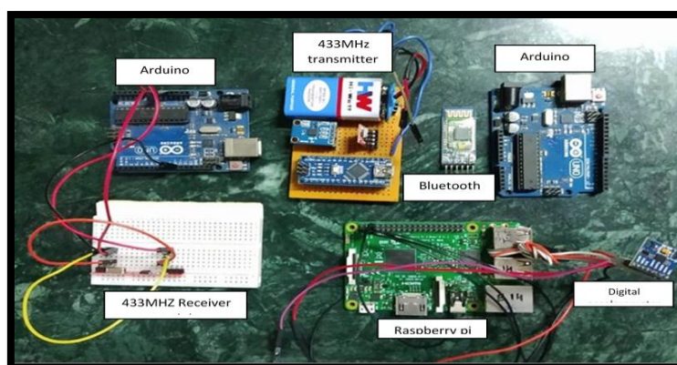
Fig.3. Wireless DAQ system components
