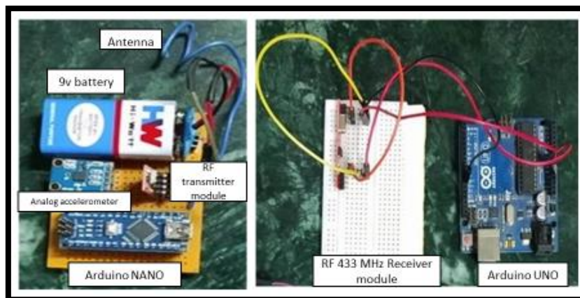
Fig.5. Wireless DAQ schememodules ofTx and Rx
