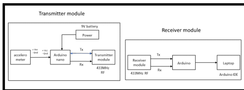
Fig.2. Block interpretation of Wireless DAQ system
